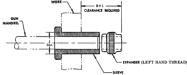
SLEEVE AND EXPANDER ASSEMBLED ON MANDREL, INSERTED INTO WORK, READY TO SET.
