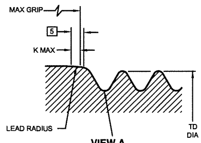
VIEW A HI-LITE THREAD TRANSITION AREA. THIS AREA OF SPECIAL CONFIGURATION AND COLD WORKING TO MEET PHYSICAL REQUIREMENTS. SEE SPECIFICATION FOR INSPECTION.
