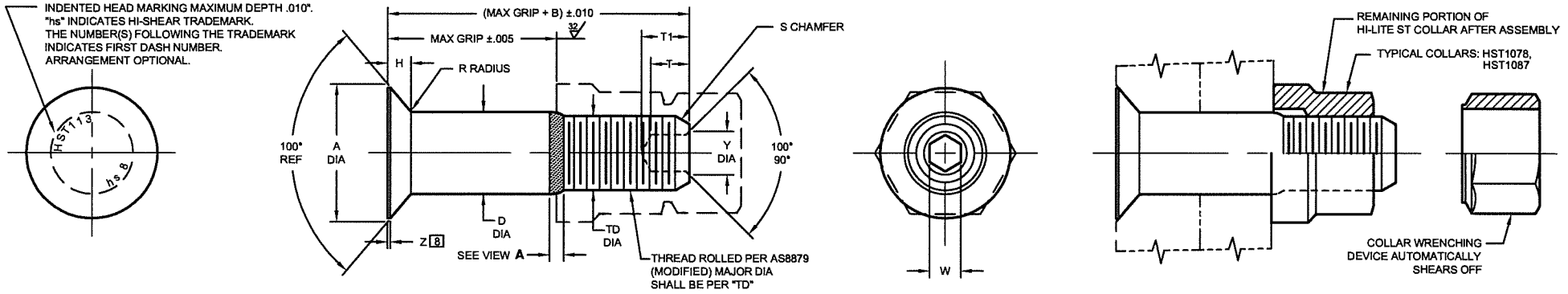
HI-LITE ST PIN AND COLLAR AFTER ASSEMBLY
